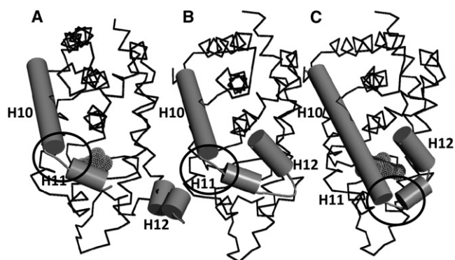
Figure 5. Comparison of CAR LBD Structures
