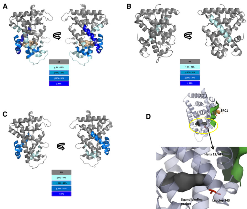
Figure 3. Perturbations in HDX Data for CAR and RXR LBDs
