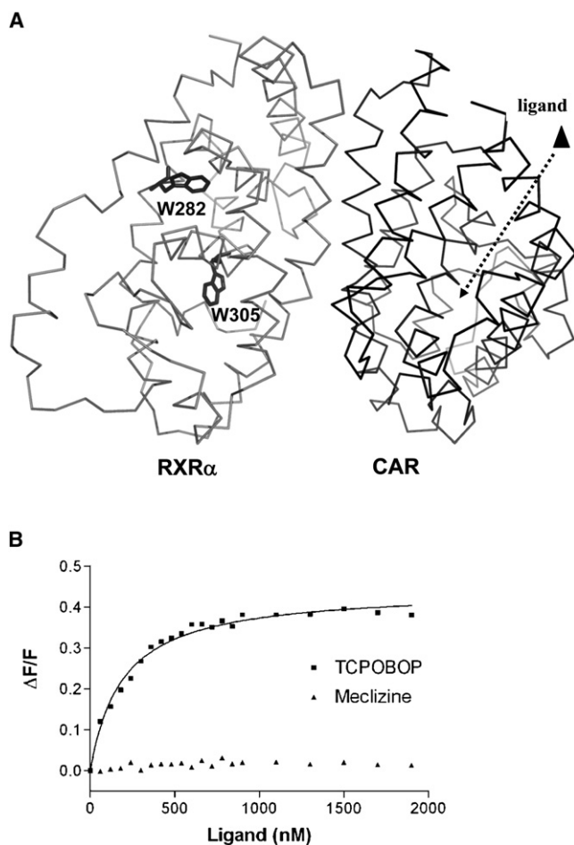
Figure 2. TCPOBOP Binding to CAR Results in a Conformational Change in RXR
