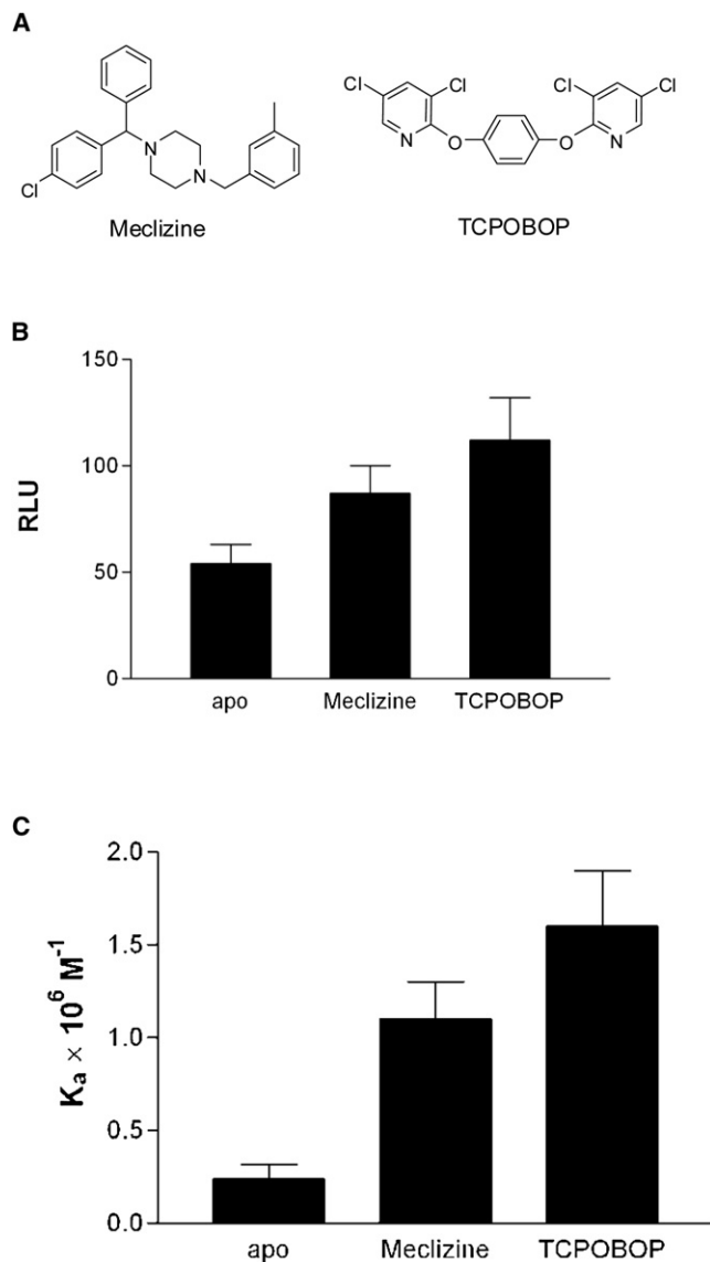
Figure 1. Comparison of the Two CAR Ligands Used in This Study (A) The chemical structures of CAR and TCPOBOP are shown. (B) TCPOBOP is a more potent agonist in cell-based reporter gene assays using the \beta RE response element. The data is shown in relative luciferase units (RLU). (C) TCPOBOP promotes higher affinity for coactivator than meclizine in ITC experiments.
