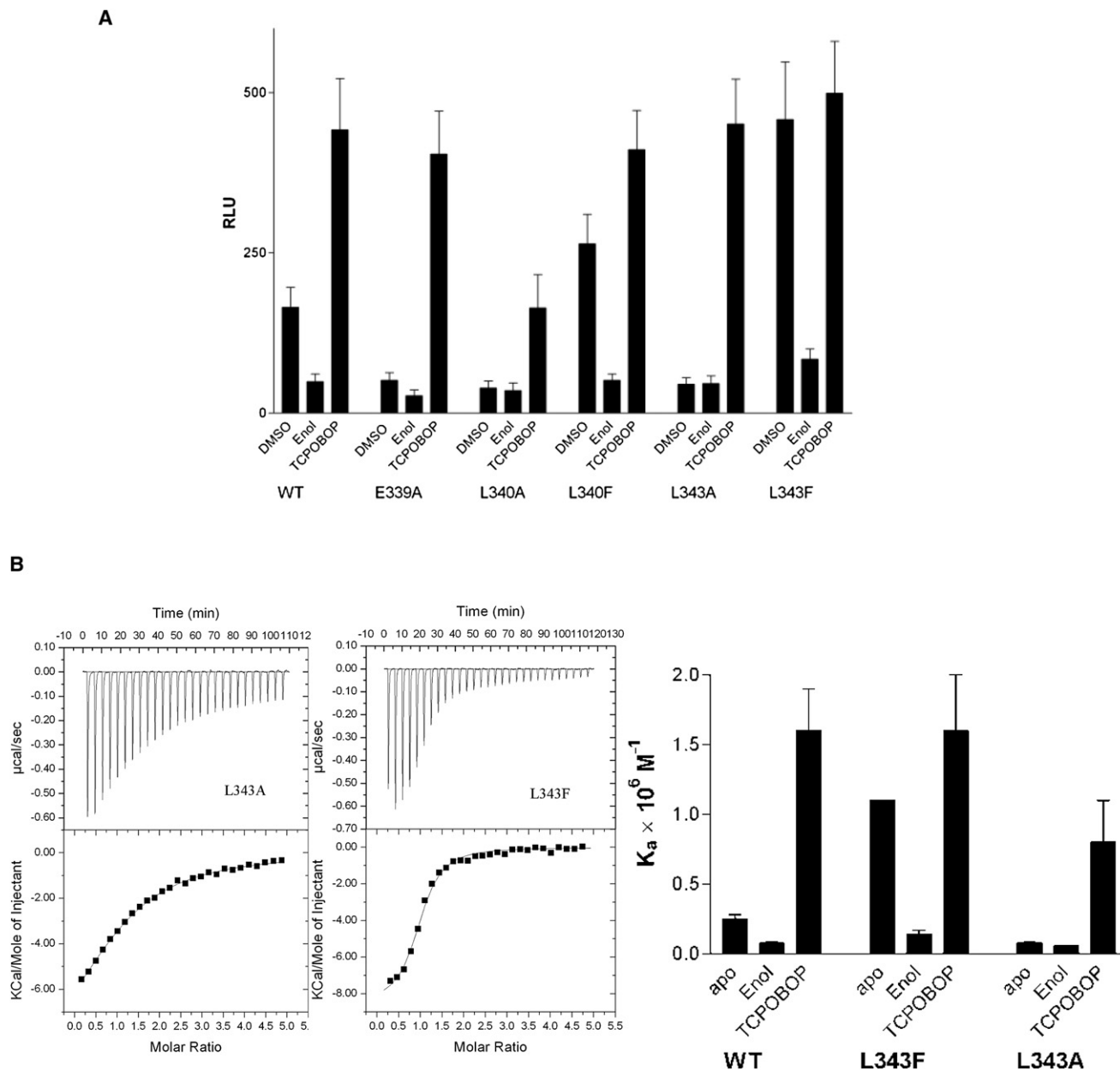
Figure 4. Transactivation and Coactivator Binding Assays of CAR:RXR
